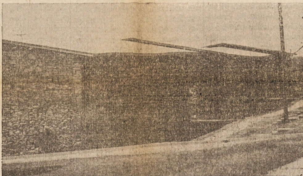
An apartment building in suburban San Antonio, Texas, shows heavy structural damage, indicated by the sagging roofline and balconies, because it was built on soils unsuitable for the type construction used. A soil survey—which can be obtained from the U.S. Department of Agriculture's Soil Conservation Service—prior to construction could have prevented costly problems. USDA PHOTO
