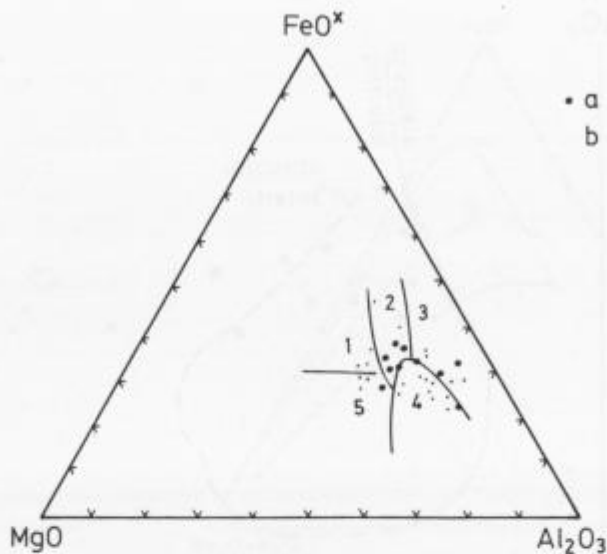
Sl. 5. Trokomponentni dijagram \text{FeOx}:\text{MgO}:\text{Al}_2\text{O}_3
