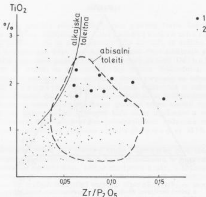
Sl. 4. Dijagram \text{TiO}_2:\text{Zr}/\text{P}_2\text{O}_5
