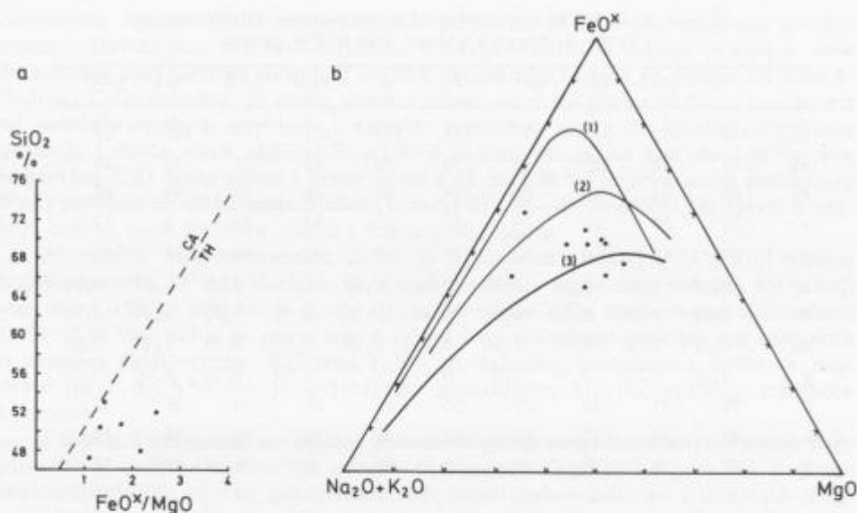
Sl. 2. a — Miyashirov dijagram \text{SiO}_2\text{:FeOx/MgO} , i b — trokomponentni dijagram \text{FeOx:Na}_2\text{O} + \text{K}_2\text{O:MgO}
