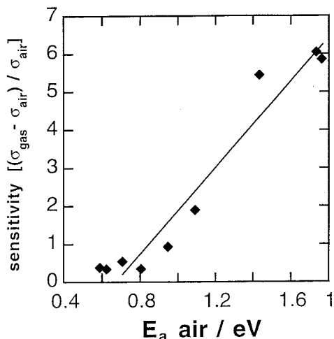
Figure 7: Correlation between E_a in air and the sensitivity to 9 ppm \text{NO}_2 , both measured at 350^\circ\text{C} , for the \text{SmFeO}_3 films tested Slika 7: Korelacija med E_a na zraku in občutljivostjo za 9 ppm \text{NO}_2 merjena pri 350^\circ\text{C} za preizkušene \text{SmFeO}_3 plasti
