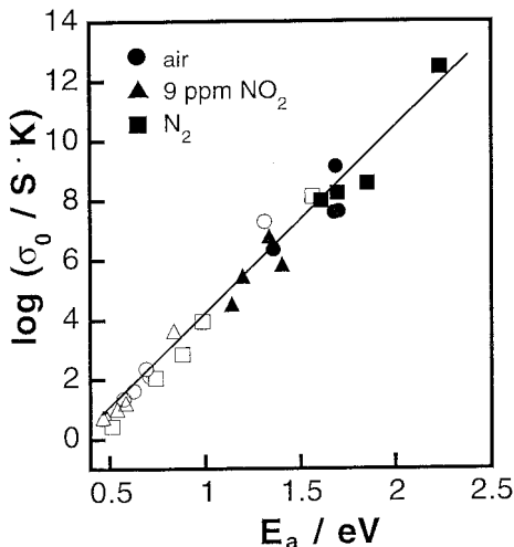
Figure 5: Correlation between E_a at 350°C and \log \sigma_0 for the SmFeO 3 films tested (close and open symbols refer to films with 4 wt% of α-terpineol or less, respectively)
