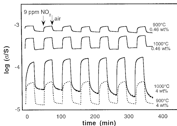
Figure 2: Electrical response at 350^\circ\text{C} of \text{SmFeO}_3 thick films prepared with different organic vehicles (0.46 and 4 wt% of \alpha -terpineol), fired at 900^\circ\text{C} and 1000^\circ\text{C} . Gas flow was changed from air to 9 ppm \text{NO}_2 in air
