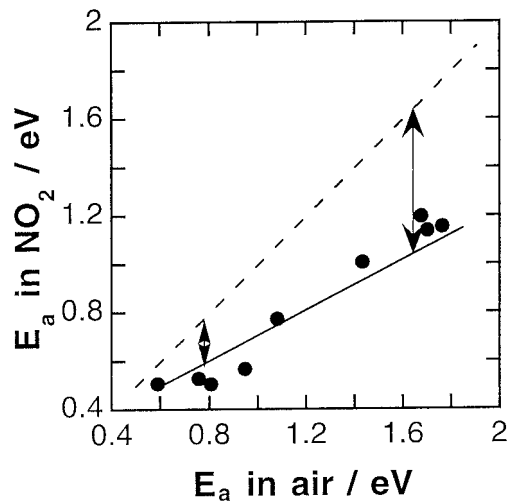
Figure 6: Correlation between the activation energies in air and 9 ppm NO 2 , measured at 350°C, for the SmFeO 3 films tested
