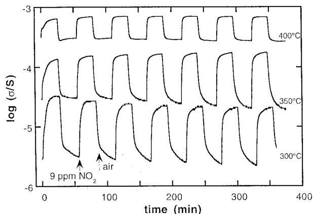
Figure 1: Electrical response at various temperatures of the \text{SmFeO}_3 thick films fired at 1000^\circ\text{C} , with 4 wt% of \alpha -terpineol. Gas flow was changed from air to 9 ppm \text{NO}_2 in air
