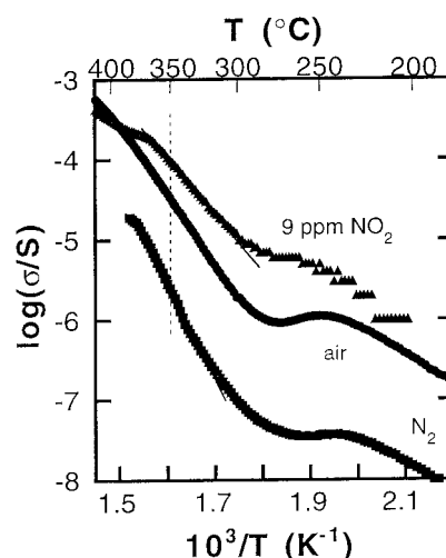
Figure 3: Temperature dependence of the conductivity for the \text{SmFeO}_3 thick films fired at 1000^\circ\text{C} with 4 wt% of \alpha -terpineol, in different gaseous atmospheres
