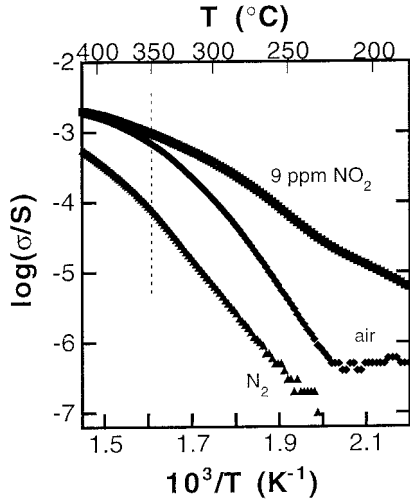
Figure 4: Temperature dependence of the conductivity for the SmFeO 3 thick films fired at 900°C with 0.46 wt% of α-terpineol, in different gaseous atmospheres
