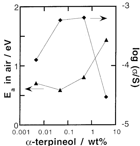
Figure 8: Correlation between the electrical properties ( E_a and conductivity) measured at 350^\circ\text{C} in air, and the content of \alpha -terpineol for the \text{SmFeO}_3 films fired at 900^\circ\text{C}
