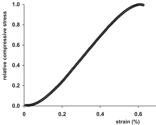
Fig. 1. A representative curve that describes the relative compressive stress with respect to strain for the used samples
