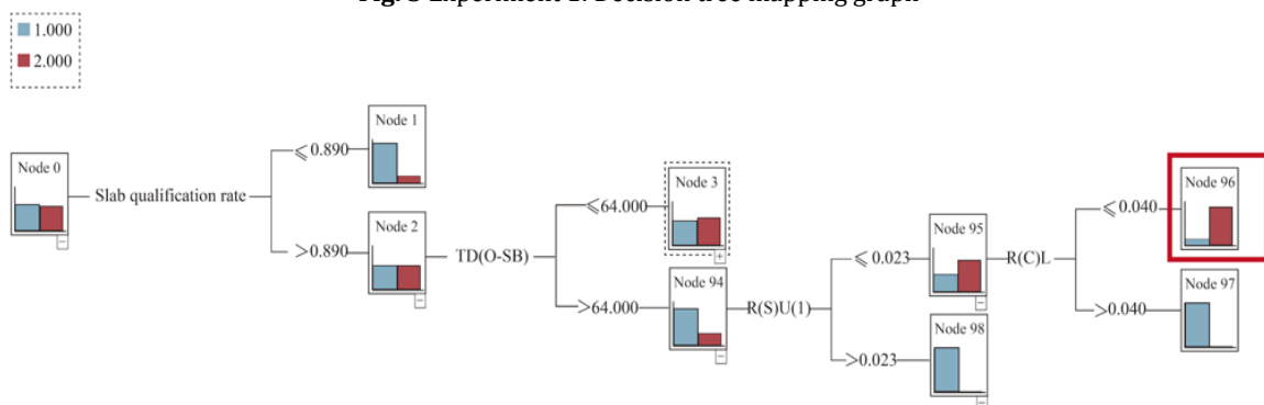
Fig. 6 Details of the decision tree for node 96
