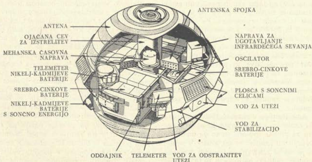
Prerez skozi satelit Transit 1 B
