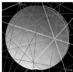
Figure 10: Specimen cooled in lead bath from 1250 °C. Microstructure: coarse-grained bainite. Microfractography, diffraction lines, resolved diffraction lines and space-orientation indexes for the marked cleavage facet
