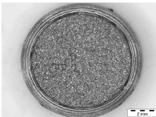
Figure 6: Fracture surface of a notched tensile specimen quenched in water from 920 °C and reheated at 750 °C. Microstructure: tempered primary fine grained martensite and secondary martensite
