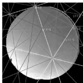
Figure 9: Specimen quenched in water from 1250 °C. Microstructure: coarse-grained martensite. Microfractography, diffraction lines, resolved diffraction lines and space-orientation indexes for the marked cleavage facet
