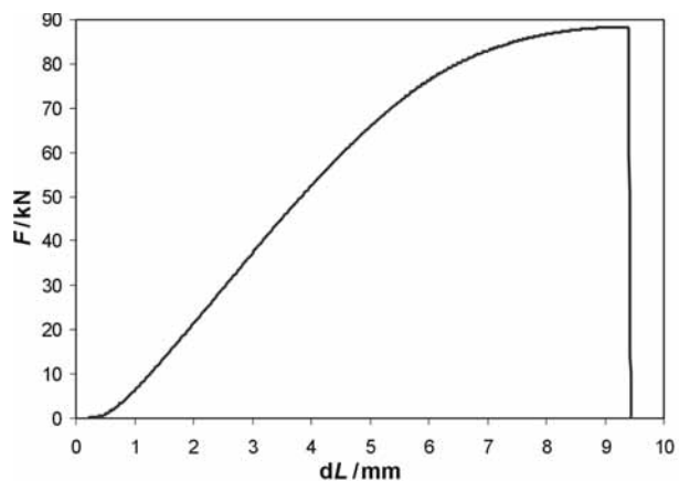
Figure 3: Dependence of force vs. extension for a specimen quenched in water from 920\text{ }^{\circ}\text{C} (a). Microstructure: fine-grained martensite
