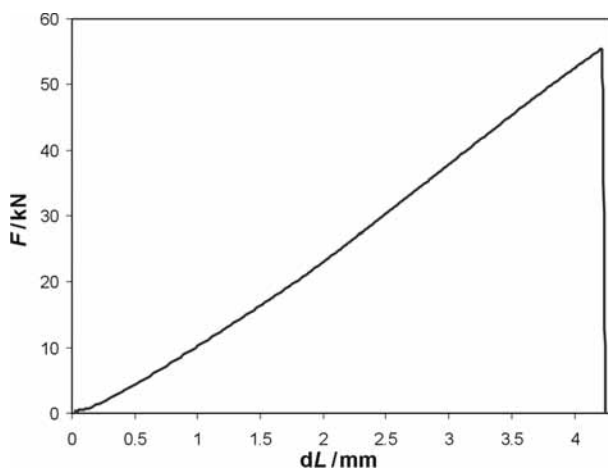
Figure 1: Dependence of force vs. extension for a specimen quenched from 1250\text{ }^{\circ}\text{C} and reheated at 750\text{ }^{\circ}\text{C} . Microstructure: coarse-grained tempered primary martensite and secondary martensite.
