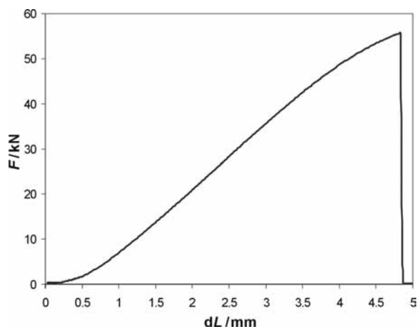
Figure 2: Dependence of force vs. extension for the specimen quenched from 1250\text{ }^{\circ}\text{C} in a lead bath at 400\text{ }^{\circ}\text{C} and reheated at 750\text{ }^{\circ}\text{C} . Microstructure: coarse-grained bainite and secondary martensite
