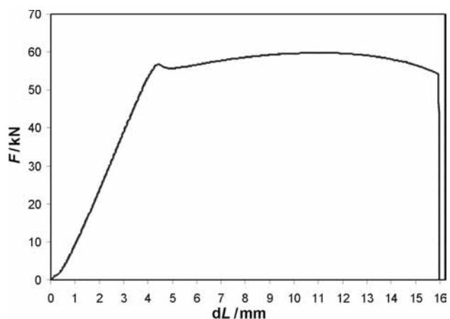
Figure 4: Dependence of force vs. extensions for a specimen with the initial microstructure reheated at 750\text{ }^{\circ}\text{C} . Microstructure: fine-grained tempered martensite–ferrite and secondary martensite
