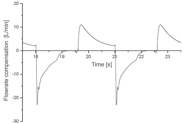
Fig. 7. The flowrate compensation effect in a variable-speed drive based on energy regulation
