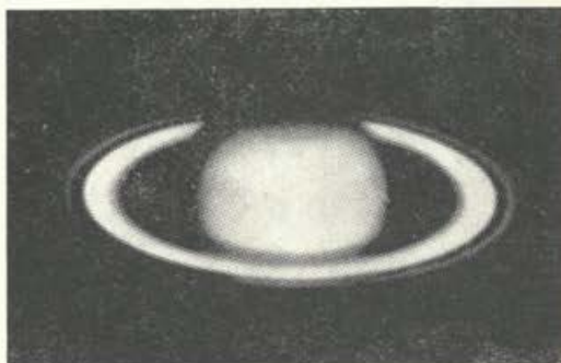
Sl. 10 Planet Saturn
