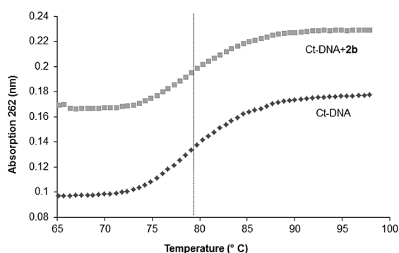
FIGURE 3. DNA as possible target of compound 2b. Thermal denaturation curves of ct-DNA ( c(\text{ct-DNA}) = 2 \times 10^{-5} \text{ M} , r_{[\text{compound}]/[\text{ct-DNA}]} = 0.3 ) at pH 7.0 (sodium cacodylate buffer, I = 0.05 \text{ M} ) upon addition of compound 2b. Error in T_m values: \pm 0.5^\circ\text{C} .
