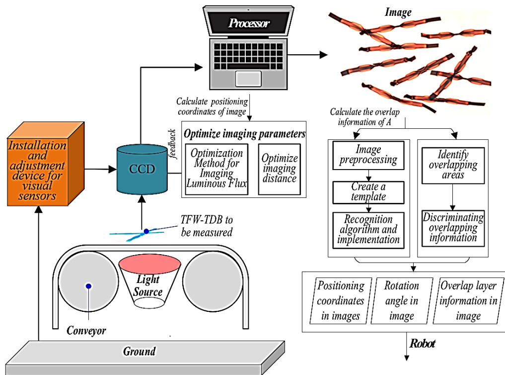
Fig. 1 Schematic diagram of TFW-TDB visual recognition system
