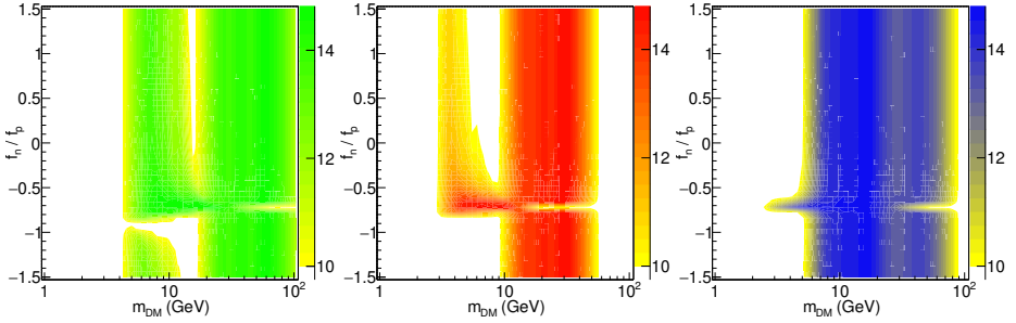
Fig. 1.3. Regions in the f_n/f_p vs m_{\text{DM}} plane allowed by DAMA experiments in the case of a DM candidate having isospin violating SI interaction. The Na and I quenching factors are: Q_I [left (green on-line)], Q_{II} [center (red on-line)], and with channeling effect [right (blue on-line)]. The considered halo is A0 (isothermal sphere) with the v_0 and \rho_0 in the range of Table III of Ref. [20]. The three possible sets of parameters A, B and C are considered (see Sect. 1.2). The color scales give the confidence level in units of \sigma from the null hypothesis .
