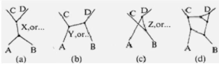
Fig. 14.1. Feynman diagrams for scatterings; Incoming particles are denoted as A and B, while intermediate ones are denoted as X, Y, Z ··· respectively.
