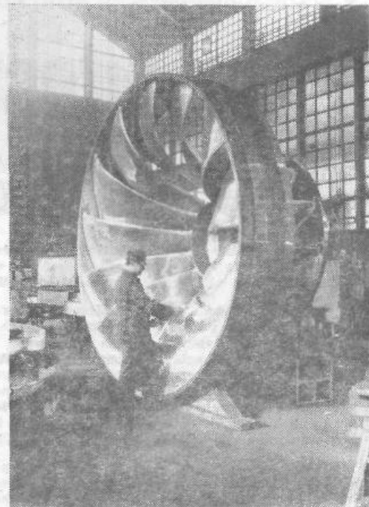
Gonilnik Francisove turbine
