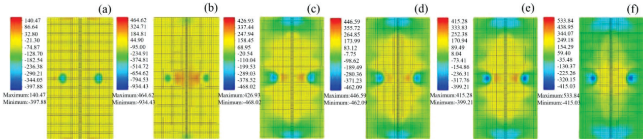
Figure 10: Numerical simulation of X-direction normal stress component under different welding parameters: a) 100 A, 11.2 V; b) 160 A, 13.6 V; c) 180 A, 14.0 V; d) 200 A, 14.3 V; e) 220 A, 14.8 V; f) 240 A, 16.2 V
