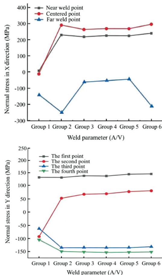
Figure 3: Trend of stress distribution: a) in the X-direction, b) in the Y-direction
