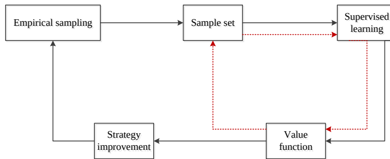
Fig. 3 Algorithm framework
