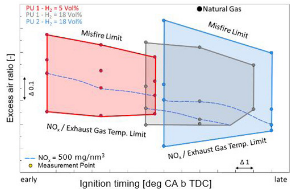
Fig. 10. Operating range of selected gas compositions
