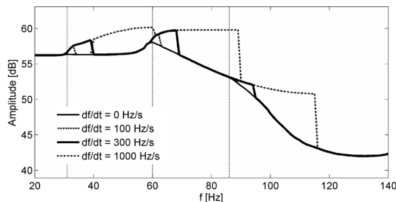
Fig. 9. Detailed time delay from Fig. 8 in frequency range 20 Hz to 140 Hz on performance delay of frequency shift
