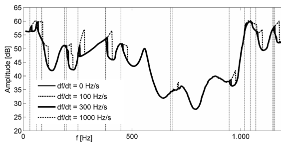
Fig. 8. Time delay of the control system is represented with frequency shift
