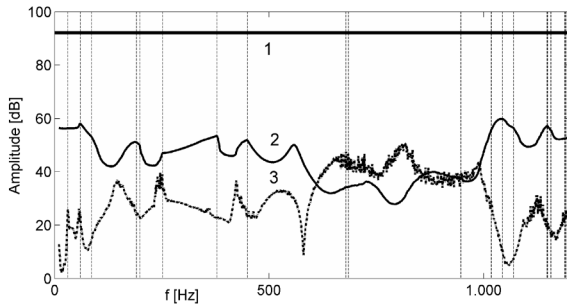
Fig. 7. Frequency response of proposed system on input signal
