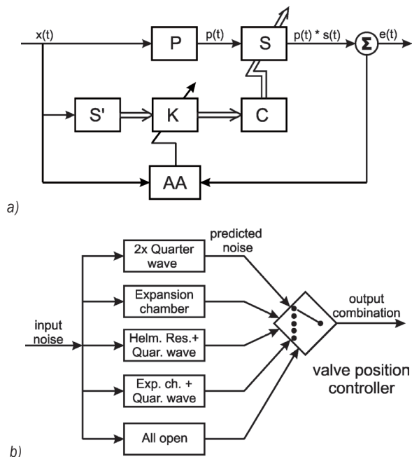
Fig. 6. Adaptive noise control principle: a) adaptive noise control algorithm, b) decision matrix
