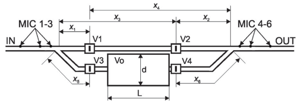
Fig. 1. Proposed adaptive muffler with active flow valves
