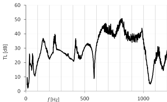
Fig. 5. Maximum overall expected TL based on measurement
