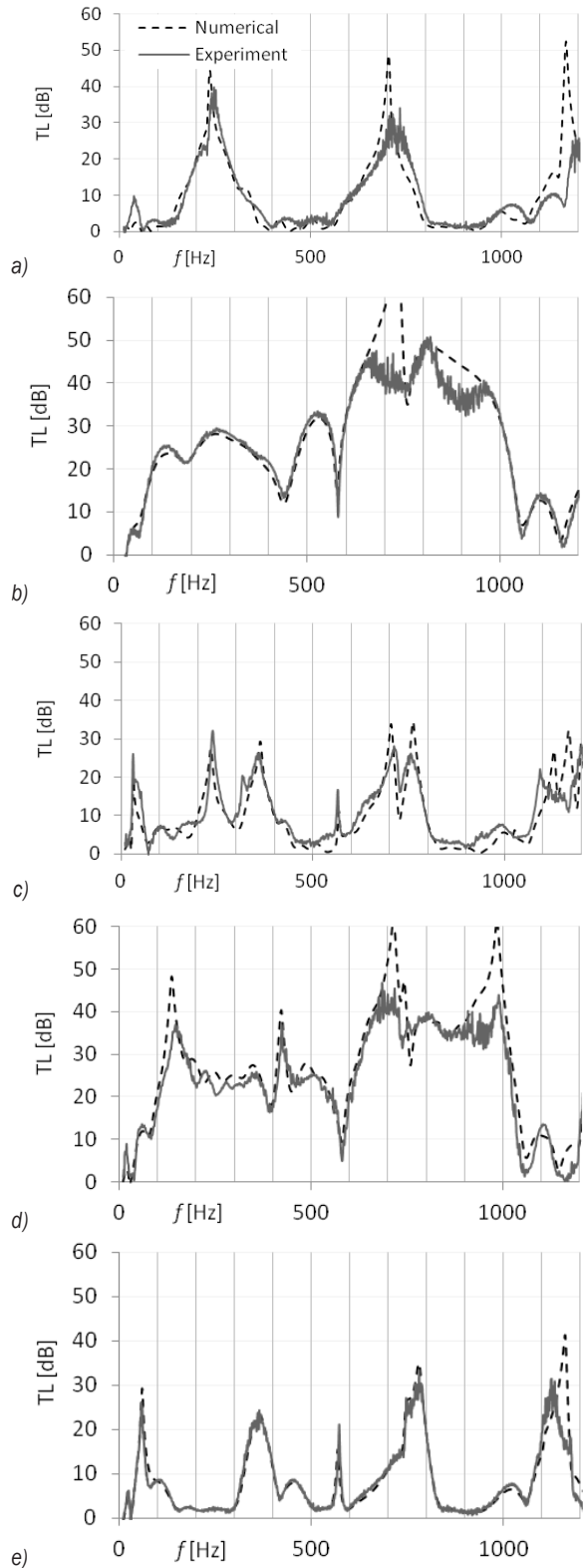
Fig. 4. Comparison between measured results and results of FEM analysis a) double \lambda/4 resonator, b) expansion chamber, c) Helmholtz resonator with \lambda/4 resonator, d) expansion chamber with \lambda/2/4 resonator, e) all open valves
