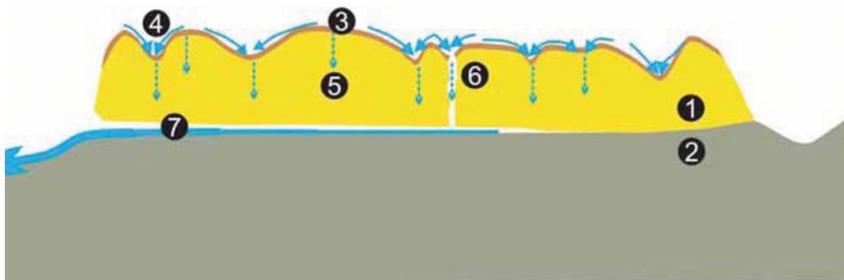
Shematski prerez terase z jamo ob stiku med konglomeratom in neprepustno podlago. Schematic cross section of a terrace with a cave at the contact between conglomerate and impermeable base.
