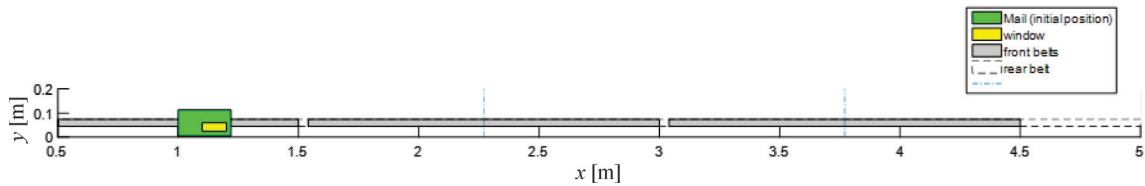
Fig. 7. Representation of the mail sorting machine with the parameters of Table 1
