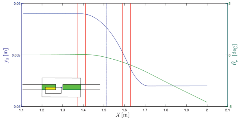
Fig. 9. Envelope vertical position and angle q_p while passing through a direction switch
