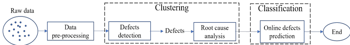
Fig. 2 Methodology Framework
