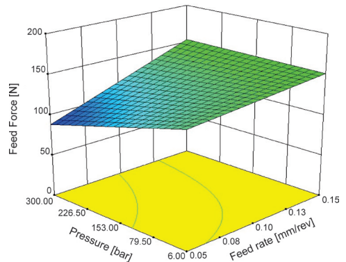
Fig. 4. Effect of pressure and feed rate on the passive force F_p ( a_p = 0.5 mm, V_c = 50 m/min)
