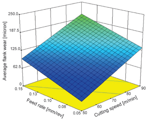
Fig. 5. Effect of cutting speed and feed rate on average tool flank wear ( a_p = 1\text{ mm} , p = 300\text{ bar} )
