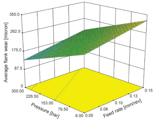
Fig. 6. Effect of coolant pressure and feed rate on average tool flank wear ( a_p = 1\text{ mm} , V_c = 90\text{ m/min} )
