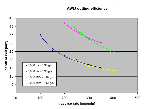
Fig. 7. Comparison of 3,500 and 6,000 bar AWIJ with used cross-over abrasive mass flow rates
