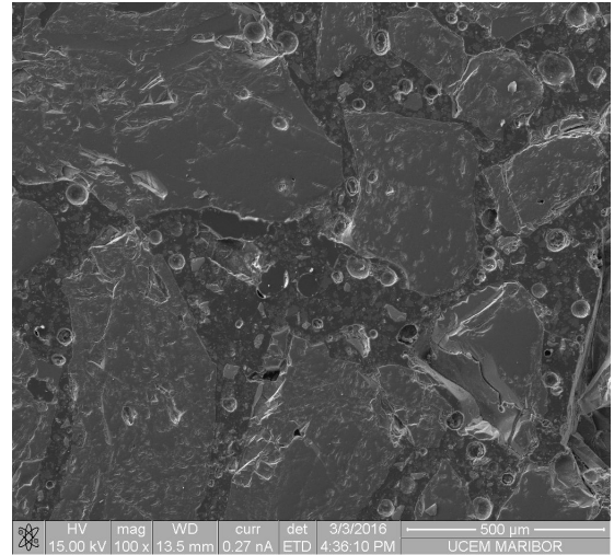
Fig. 8. Microstructure of grinding wheel sample A/07.02 [15]
