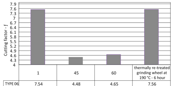
Fig. 7. Cutting factor by days for sample TYPE 06 (repeated heat processing)
