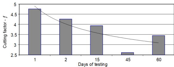
Fig. 5. Cutting factor by days for sample TYPE 02
