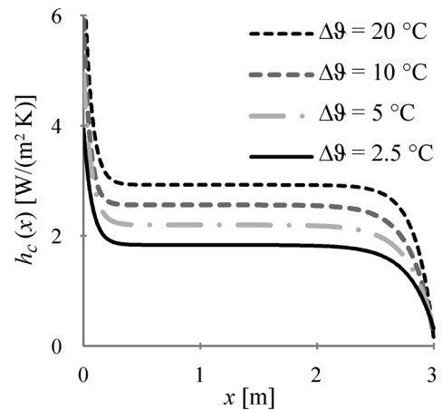
Fig. 2. Approximated local heat transfer coefficient for natural convection on TACW for temperature difference 2.5 \leq \Delta\theta \leq 20 \text{ }^\circ\text{C}
