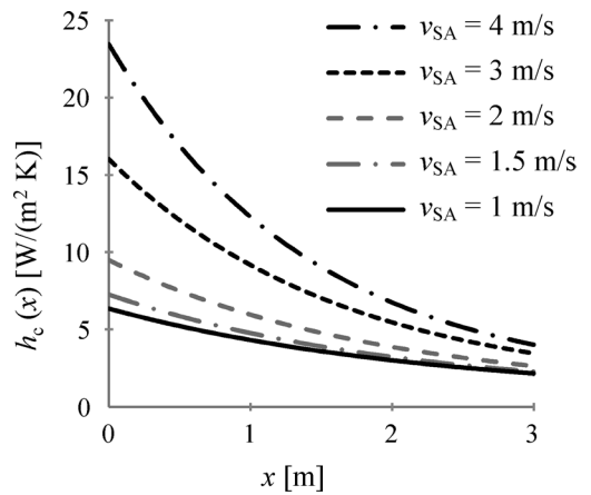
Fig. 6. Local heat transfer coefficients for mixed convection on cooled wall for 1 \leq v_{SA} \leq 4\text{ m/s} calculated due to (9)
