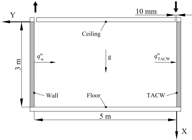
Fig. 5. Geometry of 2D office room model and boundary conditions used in numerical simulations for modeling of enhanced convection heat transfer over TACW
