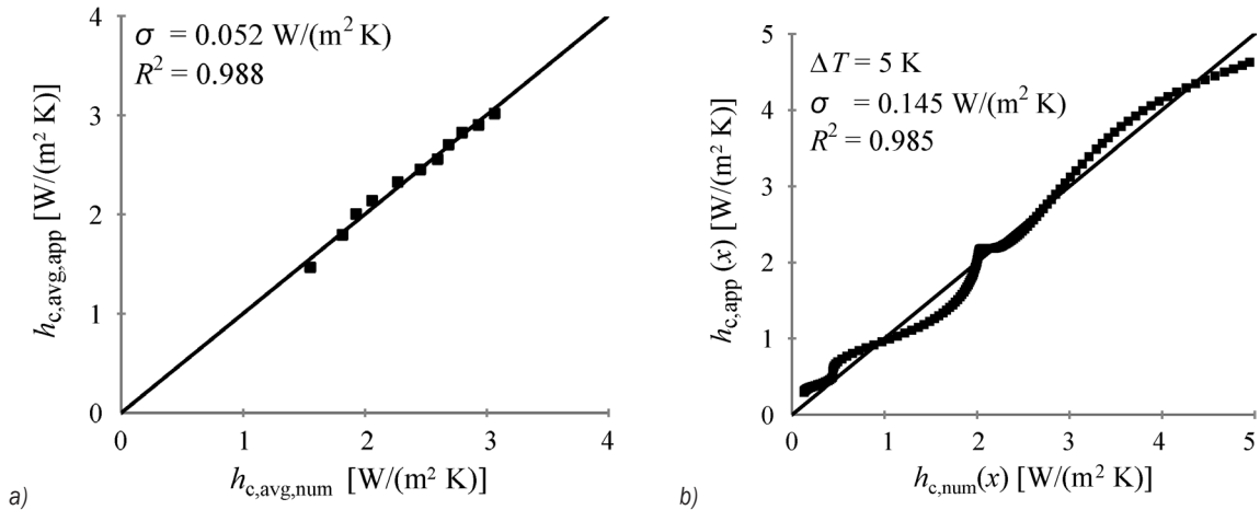
Fig. 3. Comparison between a) average h_{c,avg} and b) local h_c(x) convective heat transfer coefficient determinate by approximation function and numerical results
