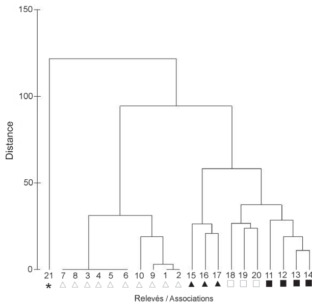
Figure 2: Dendrogram of the relevés. Enteromorpha intestinalidis-Ruppium maritima (*), Cressetum creticae (Δ), Scirpetum maritimi (▲), Puccinellio festuciformis-Sarcocornietum fruticosae (□), Juncetum maritimo-acuti (■).
