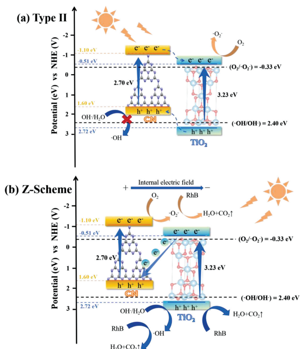
Figure 8: Mechanistic diagram of energy band structure arrangement and two possible carrier transfer mechanisms in CN/T heterojunction composites
