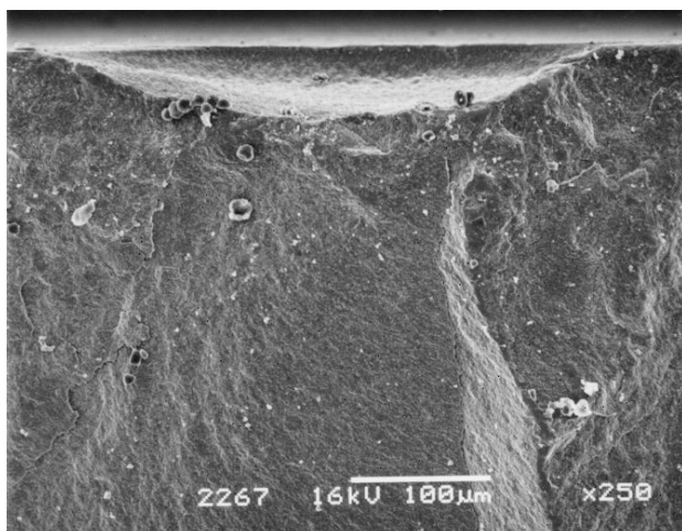
Figure 7: SEM micrograph of a fracture surface of fine-grained dry ground and sandblasted Y-TZP. Failure originated from a 50 µm deep surface pit
