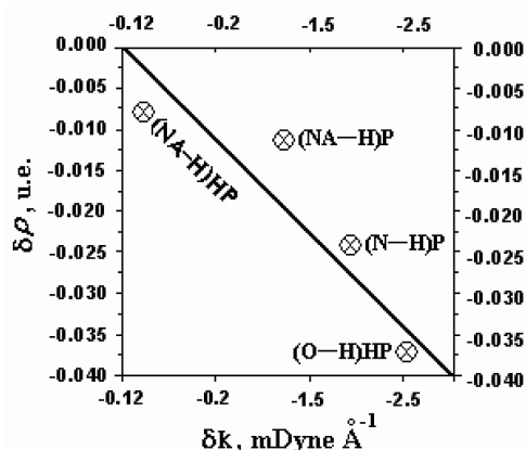
Figure 3. Relationship between the variation on the \delta k force constants and \delta\rho electronic densities of the (N–H), (O–H)HP, and (NA–H) bonds of the P\cdots(NH_3) and HP\cdots(NH_3) hydrogen bonded complexes using B3LYP/6-311++G(d,p) calculations. \delta k = -0.013\delta\rho + 0.015 , r^2 = -0.95 .
