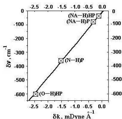
Figure 2. Relationship between the \delta\nu red-shifts and \delta k force constants of the (N-H), (O-H)HP, and (NA-H) bonds of the P\cdots(NH_3) and HP\cdots(NH_3) hydrogen-bonded complexes using the B3LYP/6-311++G(d,p) calculations. \delta\nu = 235.3\ \delta k - 11.6 , r^2 = 0.99 .
