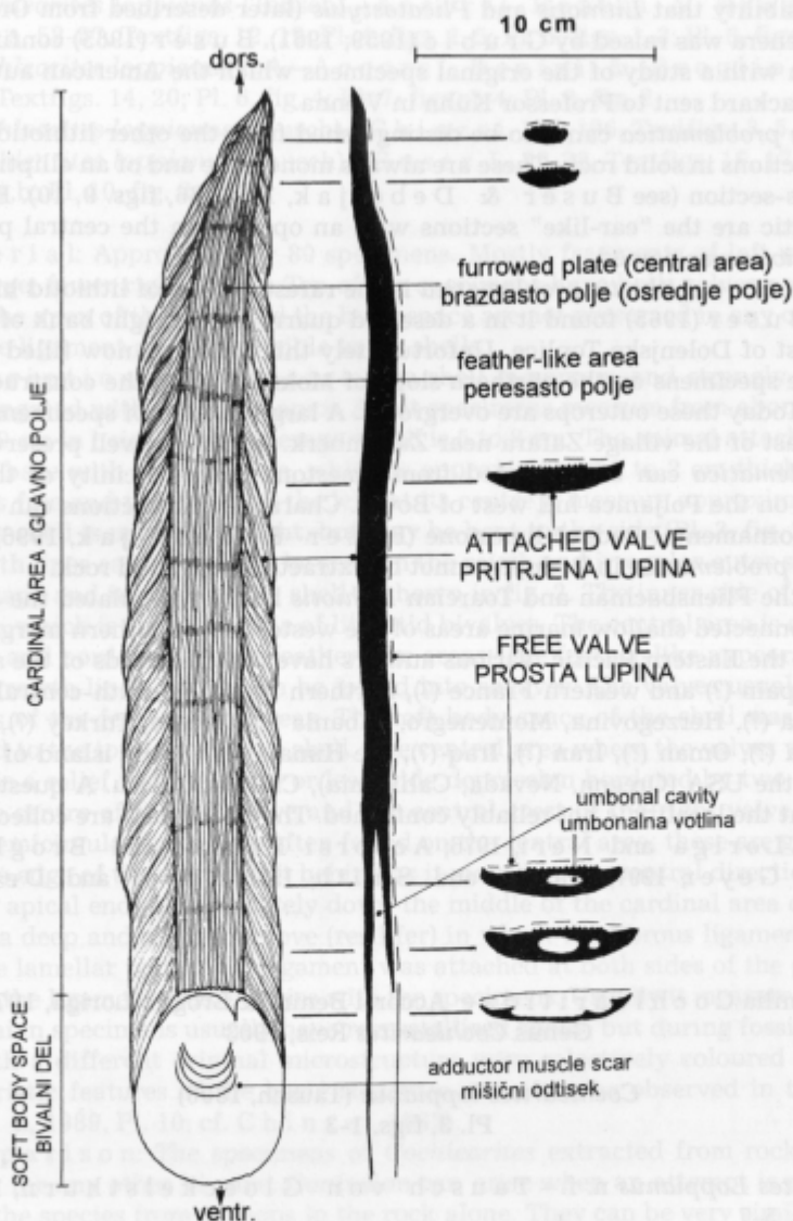
Fig. 1. Lithiotis problematica Gmbel. Left: interior side of the thicker, attached (probably right) valve. Centre: longitudinal section. Right: cross sections at various heights. The thin, free valve is marked by the dashed line. The growth position was subvertical, with the ventral end turned upwards
