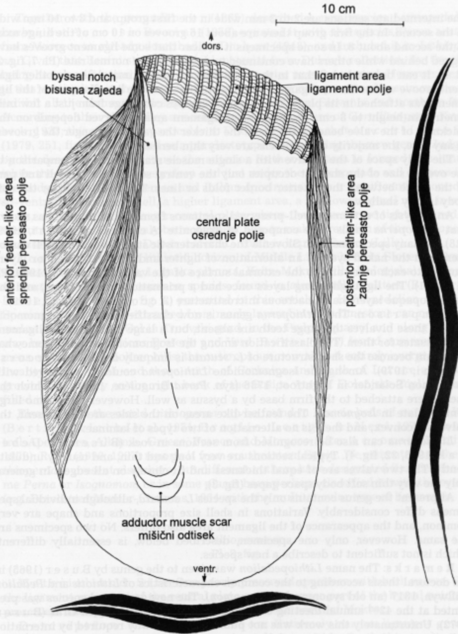
Fig. 3. Lithioperna scutata (Dubar). Left: inner surface of the right valve. Right: characteristic undulating longitudinal section of both valves. Bottom: cross sections through both valves
