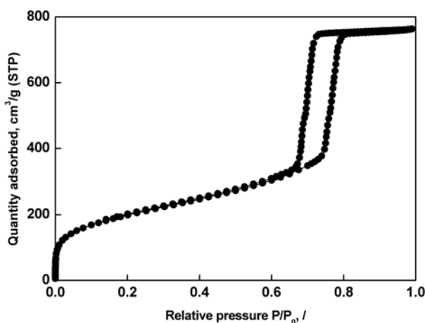
Figure 2. N 2 adsorption/desorption isotherm of the mesoporous KIT-6 silica template.
