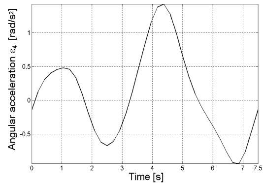
Fig. 8. Crank angular acceleration \varepsilon_4
