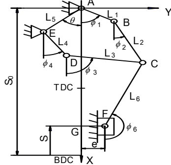
Fig. 1. Sketch of hybrid-driven press
