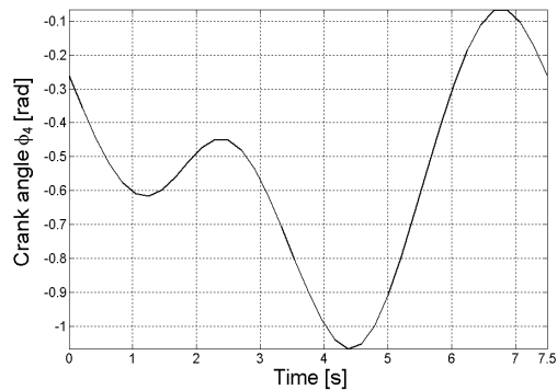
Fig. 6. Crank angular displacement \phi_4
