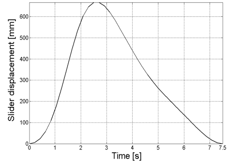
Fig. 2. Slider displacement S
