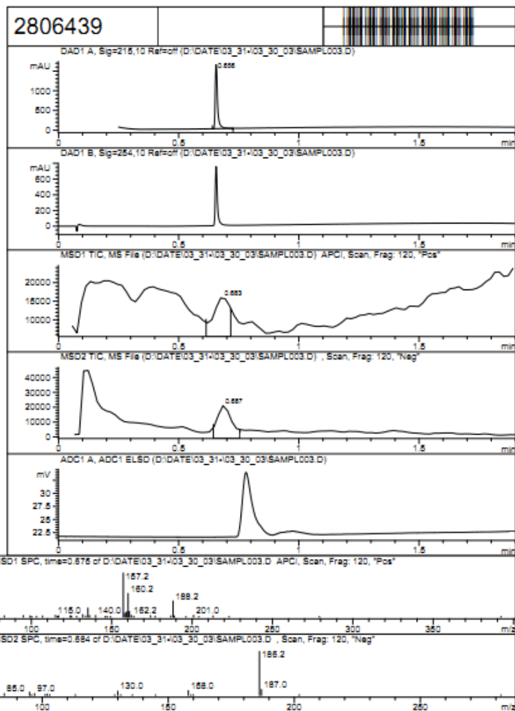
Substance 1.1 LC-MS spectrum
