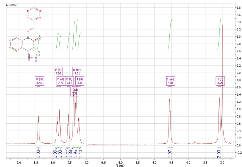
Substance 2.4 PMR spectrum
