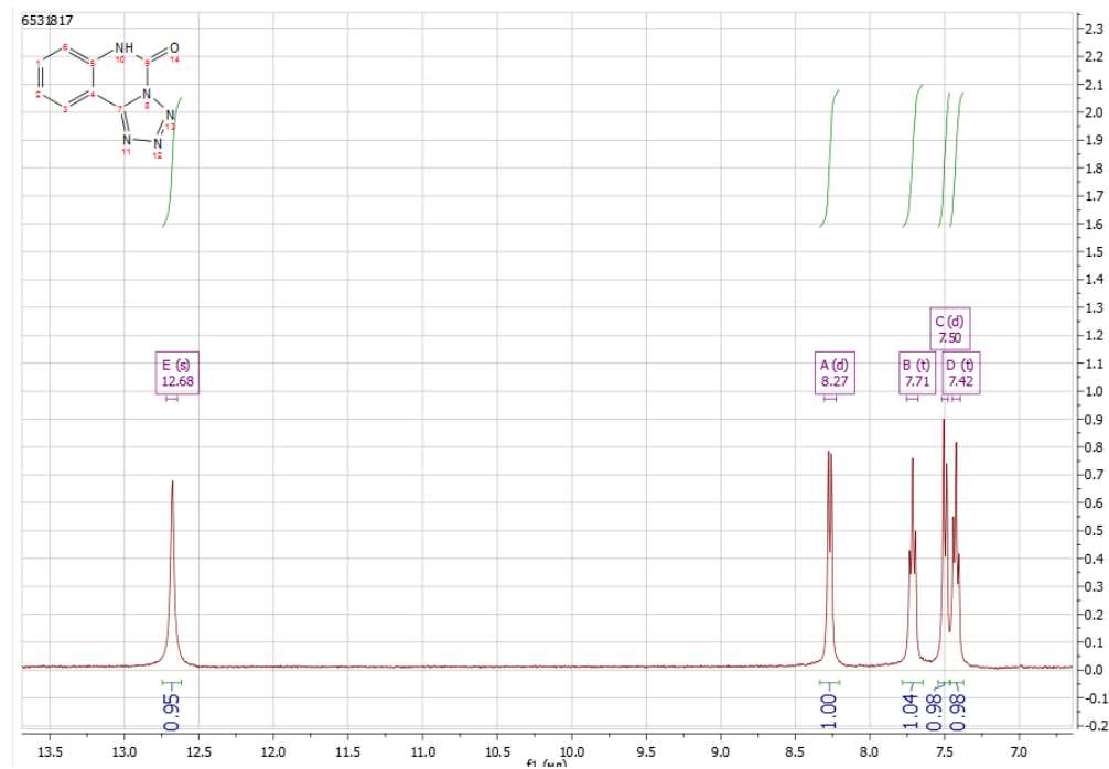
Substance 1.1 PMR spectrum
