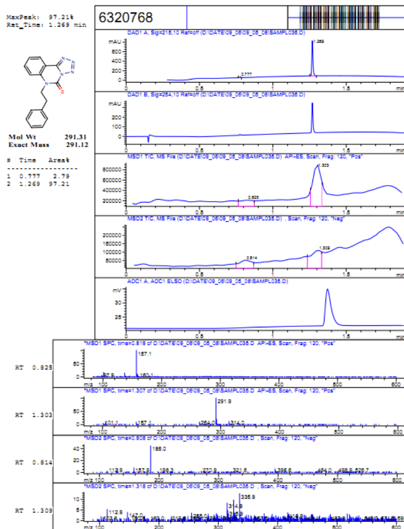
Substance 2.4 LC-MS spectrum
