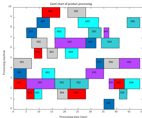
Fig. 6 Gantt chart of the optimal scheduling solution
