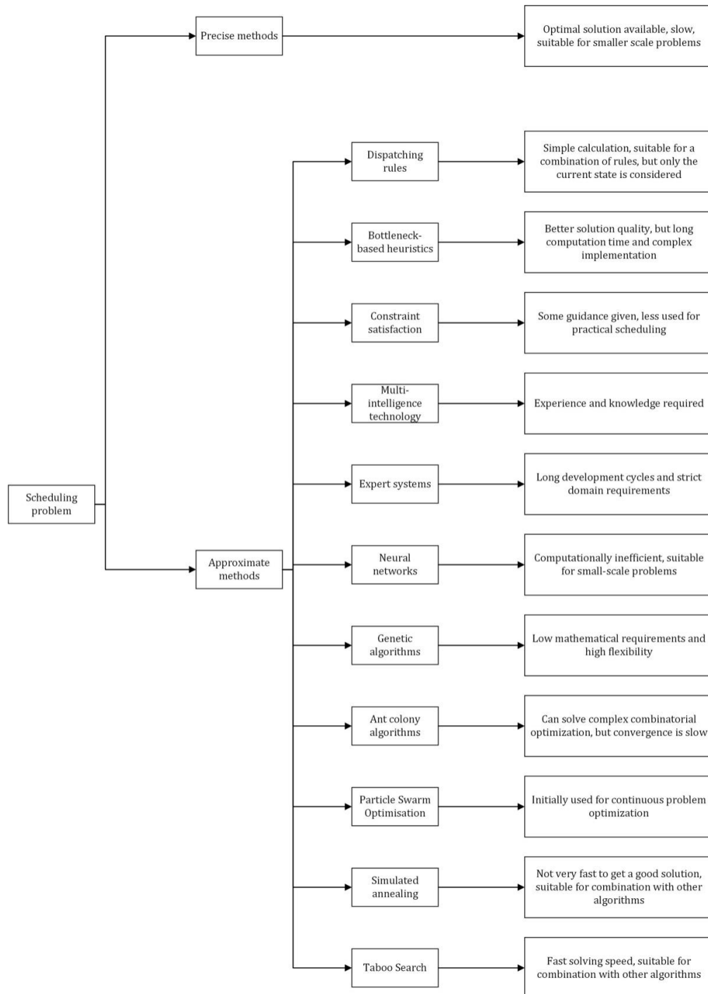
Fig. 2 Characteristics of scheduling problem solving methods
