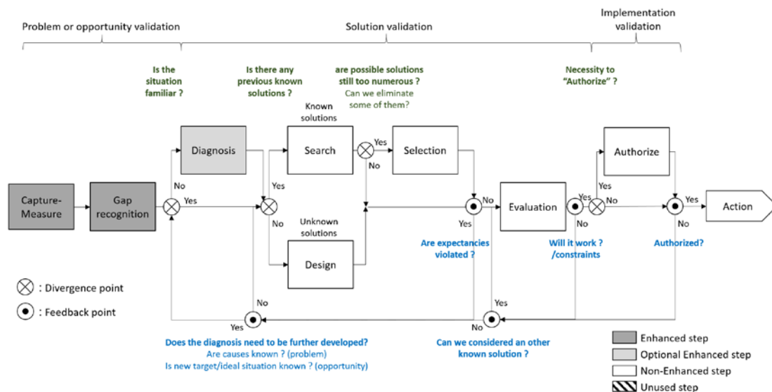
Fig. 3 Enhanced steps in the Cyber Monitoring type
