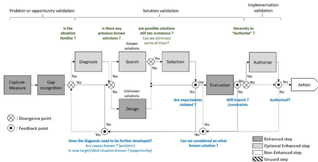
Fig. 8 Enhanced steps in the Customized Decision Support type
