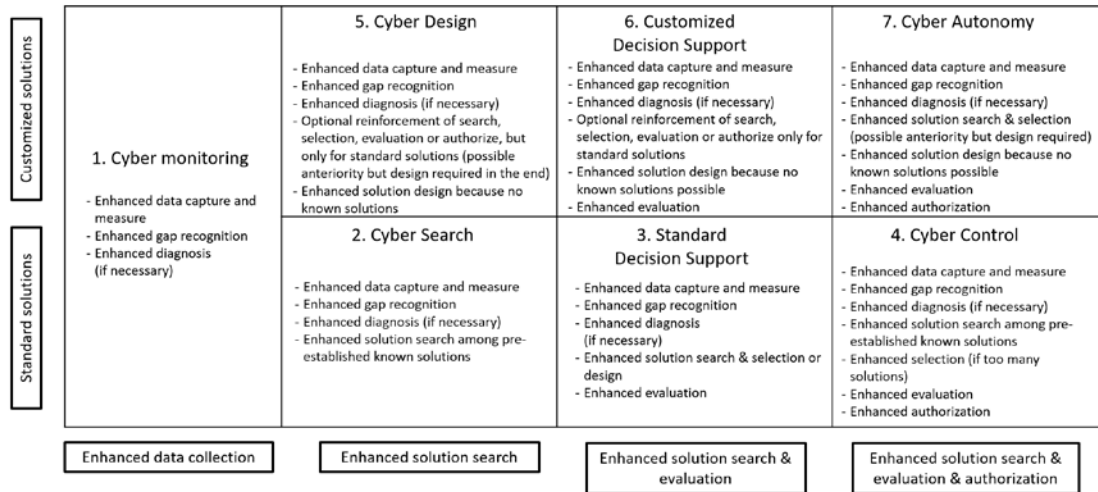
Fig. 2 Model of types of autonomy: an Industry 4.0 decision-making support model
