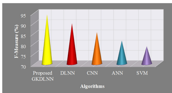
Fig. 11 F-Measure analysis
