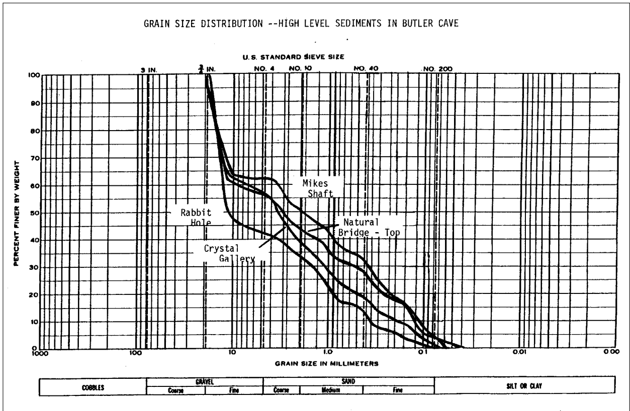
Fig. 14: Grain size distributions for various Butler Cave sediments. Sample locations are labeled on the curves. (A) Lower level sediments. (B) Upper level sediments.
