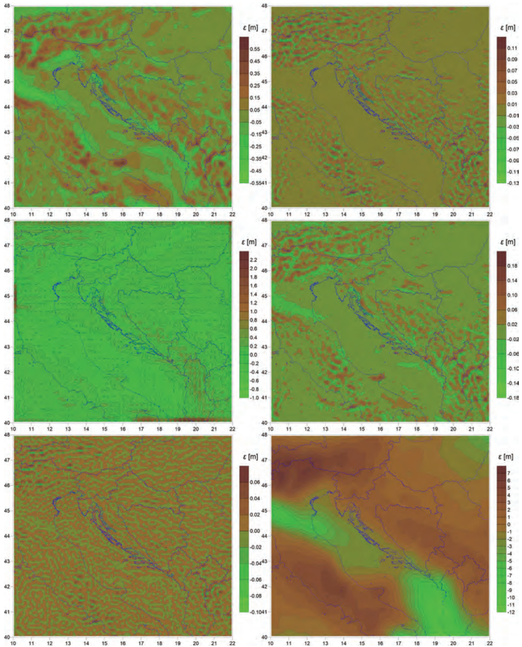
Figure 2: Contour maps showing residuals \epsilon of different methods of interpolation using GECO, from top left to bottom right: IDW, Kriging, MC, NN, RBF, MA.
