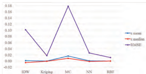
Figure 3: Comparison of RMSE, mean and median \epsilon for different methods of interpolation and GEKO model
