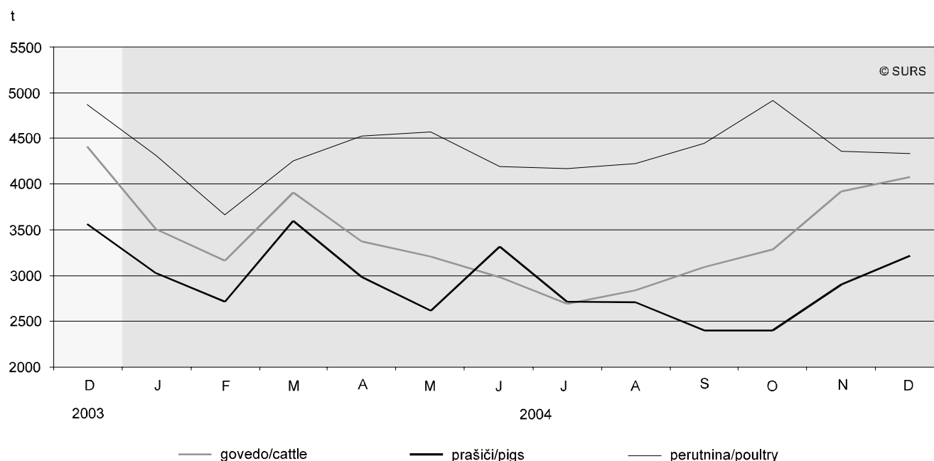
Chart 1: Weight of dressed carcass of slaughtered livestock in slaughterhouses, Slovenia, December 2003 - December 2004
