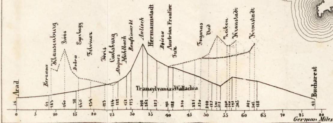
Section and Gradients of the projected line Arad-Hermannstadt to Bucharest and Kustandji.
