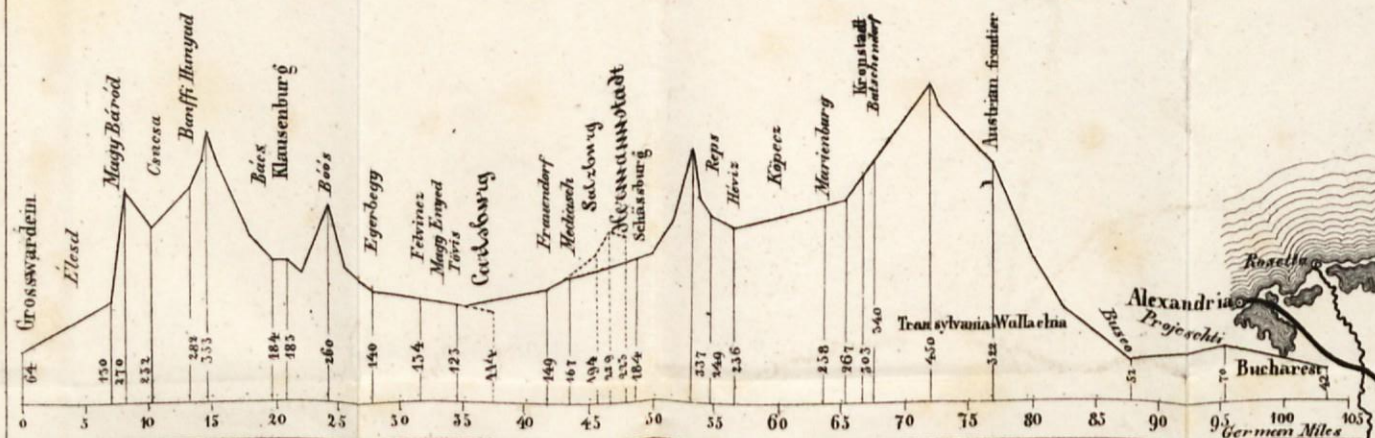
Section and Gradients of the projected line Grosswardein, Klausenburg, Kronstadt to Bucharest and Galatz.
