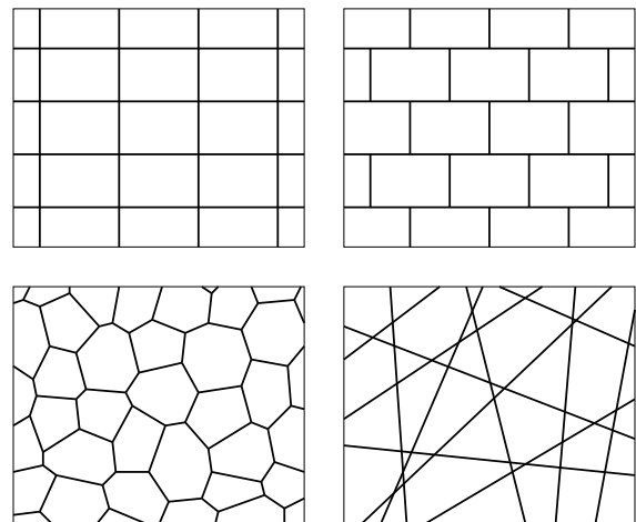
Fig. 1. Examples of planar tessellations.
