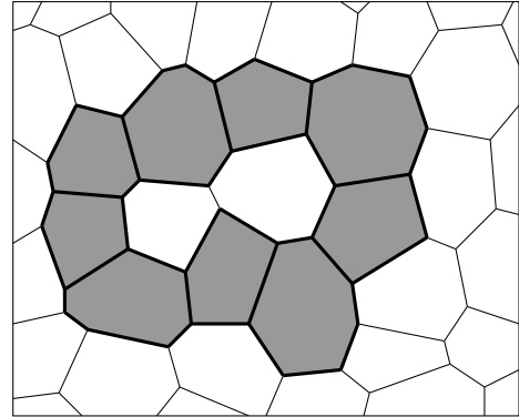
Fig. 3. If X is a union of cells, then only the facets within it need to be considered. Eq. (4) gives N(X) = 9 - 45 + 36 = 0 .
