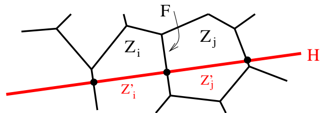
Fig. 4. Example of a tessellation induced on a hyperplane.
