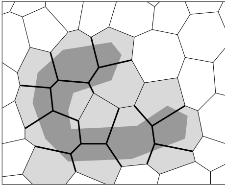
Fig. 2. Example of regional measurement. The measurement fields are the cells of the tessellation. The EPC of the dark domain is N(X) = 14 - 23 + 10 = 1 .
