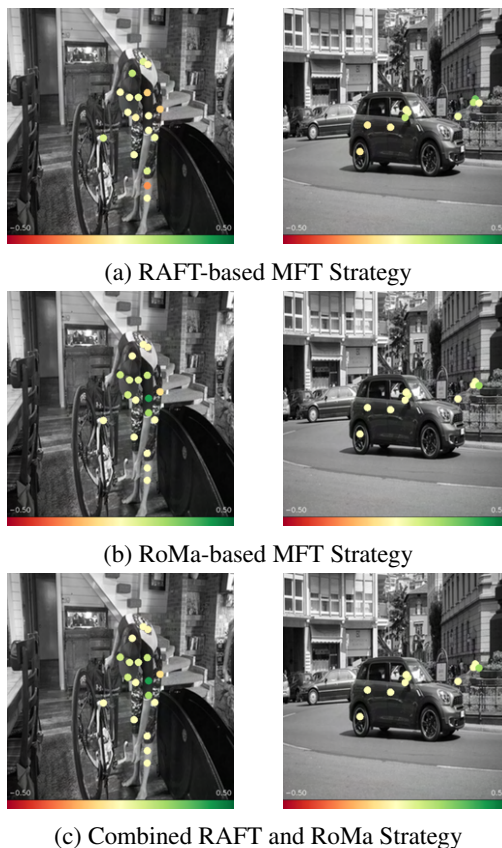
Figure 3: Images show the first frames of two selected TAP-Vid DAVIS sequences. Dots represent ground-truth tracking points, with shades of green showing the improvement in \langle \delta_{avg}^x \rangle achieved by the Selective RoMa Position Prediction ensemble over methods (a)-(c), shades of red show the converse.
