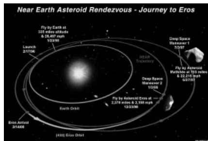
Sre{anje sonde NEAR z Erosom
