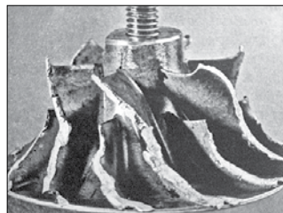
Poškodbe turbine in batov
