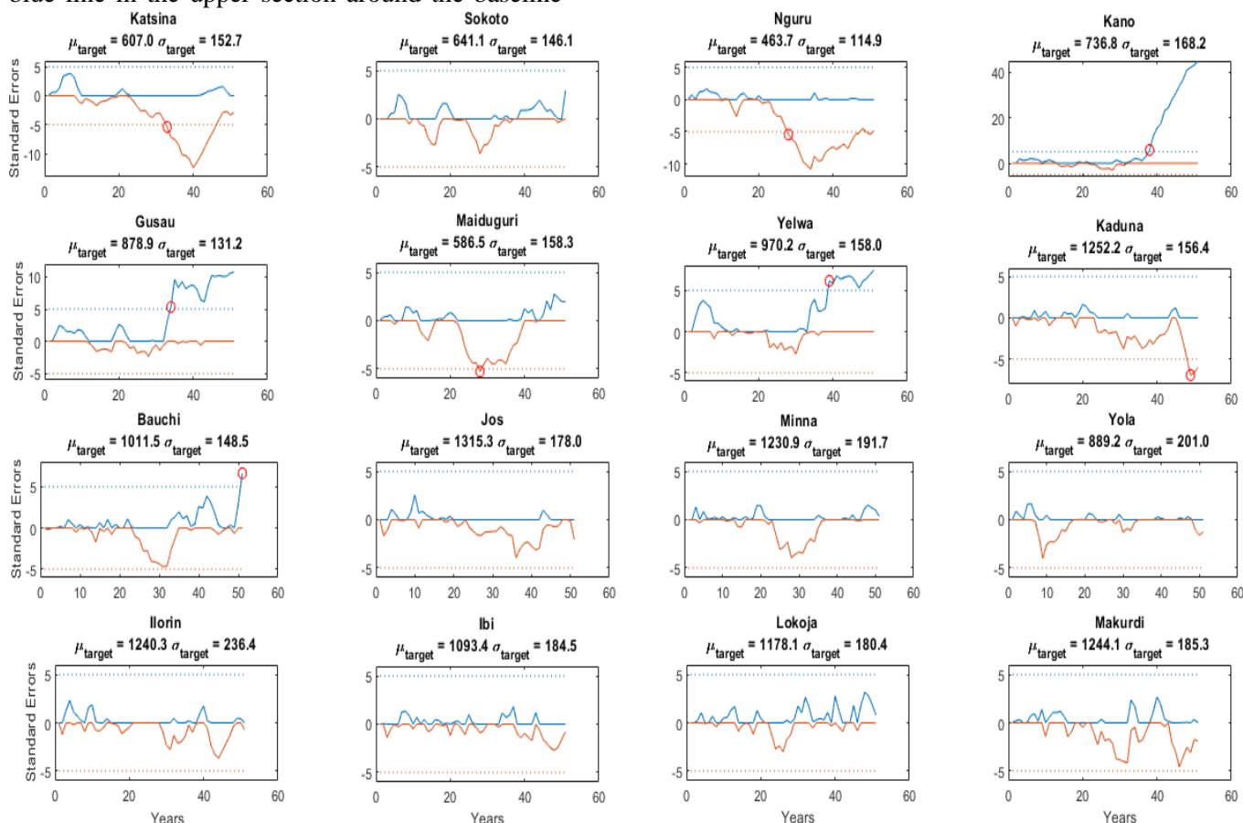
Figure 2: CUSUM plot for the northern stations in Nigeria considered in this study.
