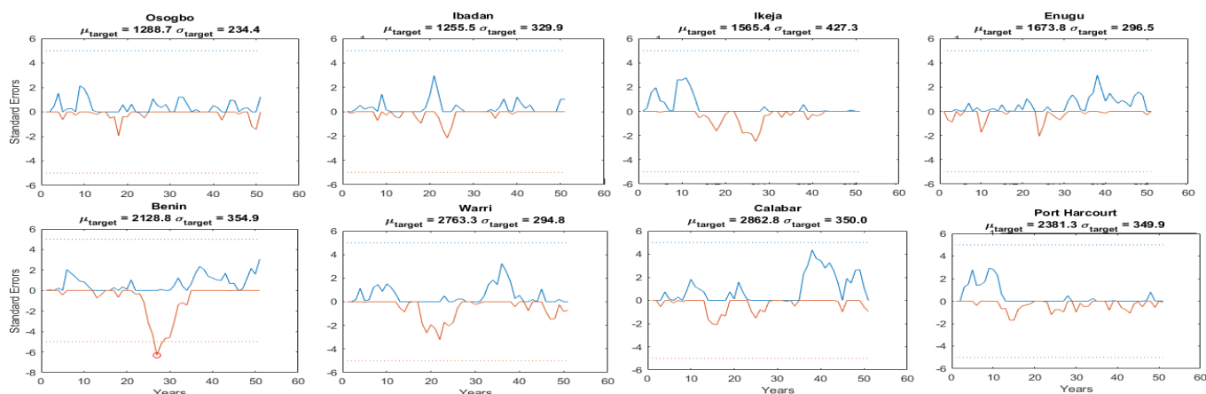
Figure 3: CUSUM plot for the southern locations in Nigeria evaluated in this study.
