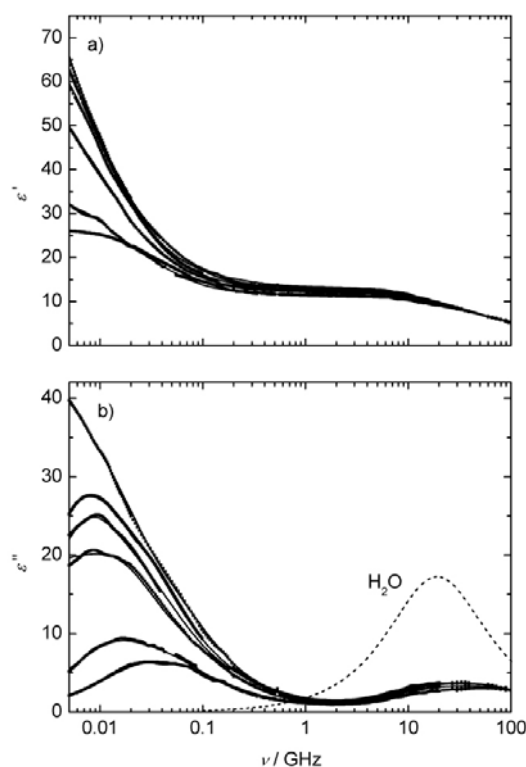
Figure 2. Dielectric permittivity, \epsilon'(\nu) (a), and loss, \epsilon''(\nu) (b), spectra for DDAB/NaBr(aq)/D microemulsions at n -dodecane mass fraction w_D = 0.35 with water/surfactant mole ratio W = 119 . NaBr concentrations: c/\text{mM} = 0, 0.05, 0.10, 0.50, 0.80, 1.0 (top to bottom). Also included in (b) is the dielectric loss spectrum of pure water, scaled to its concentration in the microemulsion system ( c_W \cdot \epsilon''/c_W^\circ ).
