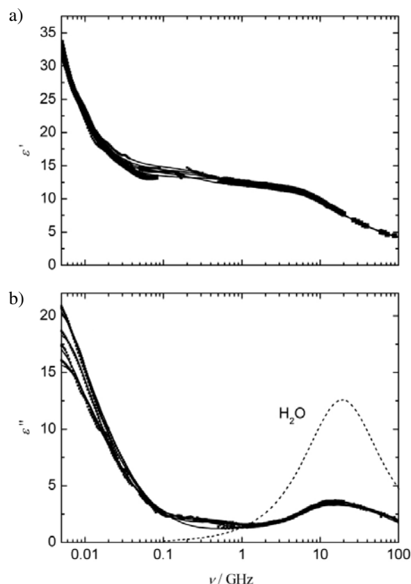
Figure 5. Dielectric permittivity, \epsilon'(v) (a), and loss, \epsilon''(v) (b), spectra for DDAB/ (CH_3)_4NBr(aq) /D microemulsions at n -dodecane mass fraction w_D = 0.35 with water / surfactant mole ratio W = 38.5 . (CH_3)_4NBr concentrations: c/mM = 0, 1.0, 5.0, 7.0, 10 (top to bottom). Also included in (b) is the dielectric loss spectrum of pure water, scaled to its concentration in the microemulsion system ( c_w \cdot \epsilon'' / c_w^\circ ).
