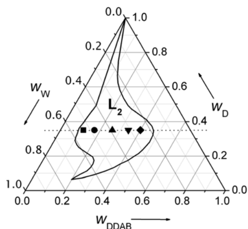
Figure 1. Phase diagram of the system DDAB/W/D at 25 ^\circ\text{C} 8 showing the microemulsion phase ( L_2 ). Samples investigated in this work were at dodecane mass fraction w_D = 0.35 and water/surfactant mole ratios of W = 119 (■), 72 (●), 39 (▲), 23 (▼), 16 (◆).
