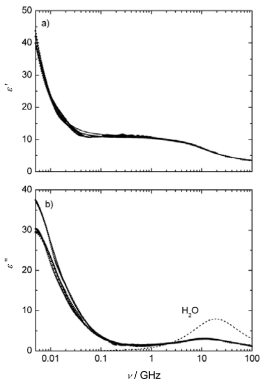
Figure 3. Dielectric permittivity, \varepsilon'(\nu) (a), and loss, \varepsilon''(\nu) (b), spectra for DDAB/NaBr(aq)/D microemulsions at n -dodecane mass fraction w_D = 0.35 with water / surfactant mole ratio W = 15.9 . NaBr concentrations: c/\text{mM} = 0, 1.0, 25 (top to bottom). Also included in (b) is the dielectric loss spectrum of pure water, scaled to its concentration in the microemulsion system ( c_w \cdot \varepsilon''/c_w^\circ ).
