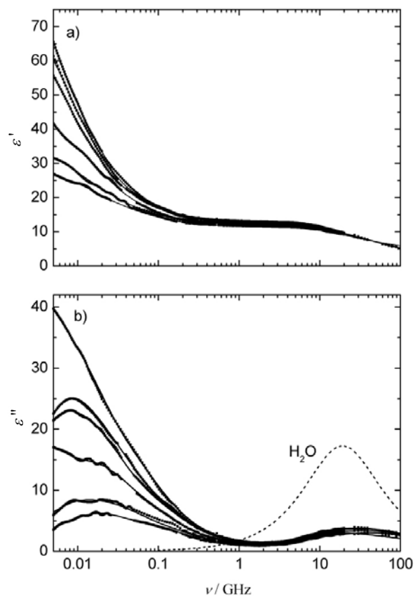
Figure 4. Dielectric permittivity, \varepsilon'(\nu) (a), and loss, \varepsilon''(\nu) (b), spectra for DDAB/(CH 3 ) 4 NBr(aq)/D microemulsions at n -dodecane mass fraction w_D = 0.35 with water / surfactant mole ratio W = 119 . (CH 3 ) 4 NBr concentrations: c/\text{mM} = 0, 0.05, 0.18, 0.50, 0.80, 1.0 (top to bottom). Also included in (b) is the dielectric loss spectrum of pure water, scaled to its concentration in the microemulsion system ( c_w \cdot \varepsilon''/c_w^\circ ).
