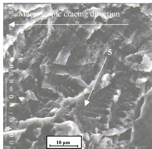
Fig. 5. “Triangles” after the tests in H_2SO_4 .
