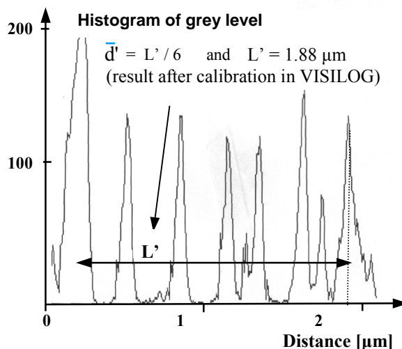
Fig. 6. Measurement of \bar{d}'_{corrected} striation spacing on histogram.
