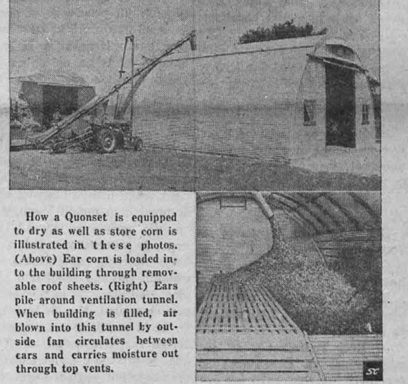
How a Quonset is equipped to dry as well as store corn is illustrated in these photos. (Above) Ear corn is loaded into the building through removable roof sheets. (Right) Ears pile around ventilation tunnel. When building is filled, air blown into this tunnel by outside fan circulates between ears and carries moisture out through top vents.
