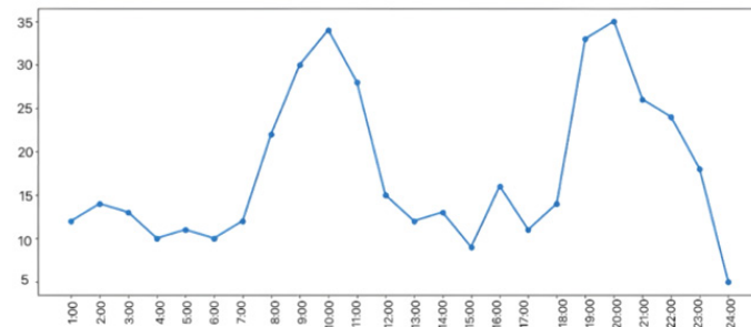
Fig. 3 Diagram of daily charging load variation at a charging station in Shanghai
