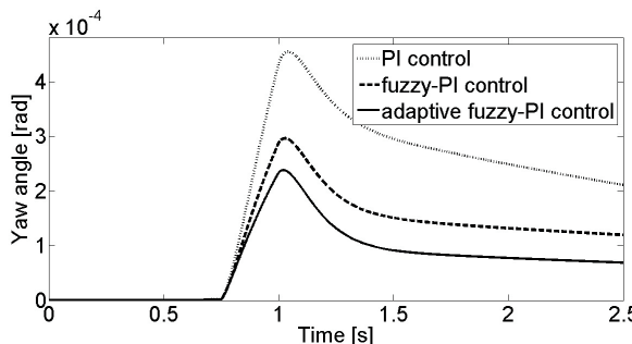
b) Firing angle of 60 degrees
