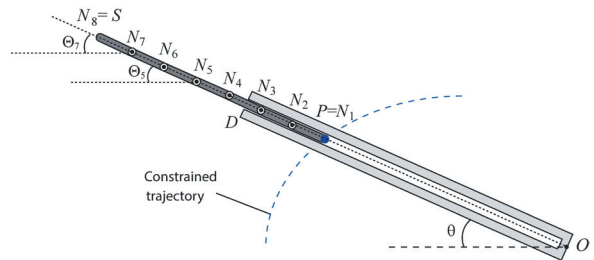
Fig. 2. Lumped mass model of the flexible link with rigid support (guide)
