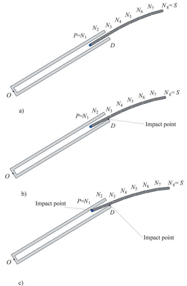
Fig. 3. Constrained flexible extensible link with rigid support and clearance model; a) no impact, b) impact on one point, and c) impact on two points
