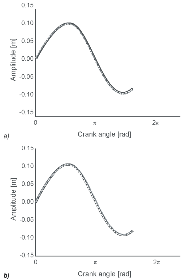
Fig. 8. Dynamic behaviour of the active end flexible manipulator with clearance along the active trajectory immediately after the quick stop, a) trajectories without; and b) with clearance for 2 (gray/dotted), 4 (black) and 9 (white/dashed) links simulation
